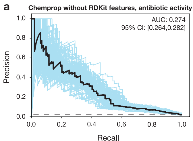
Extended Data Fig. 2 | Comparison of deep learning models for predicting antibiotic activity. a,b , Precision-recall curves for predictions of antibiotic activity, for an ensemble of 10 Chemprop models without RDKit features ( a ) and the best-performing random forest classifier model based on Morgan fingerprints ( b ), trained and tested using data from a screen of 39,312 molecules
