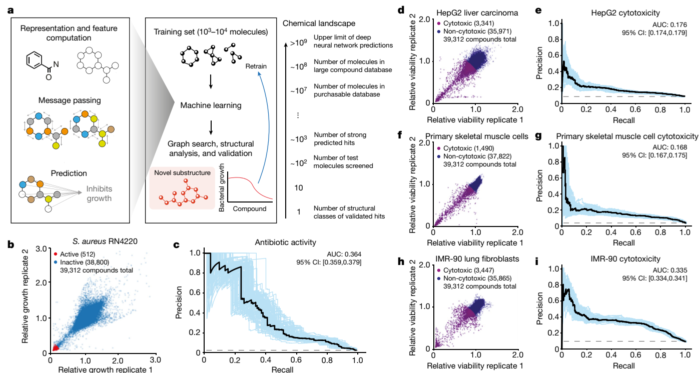
Fig. 1 | Ensembles of deep learning models for predicting antibiotic activity and human cell cytotoxicity. a , Schematic of the approach. Graph neural networks predict the chemical properties of more than 10^9 molecules in silico, in contrast to expensive and time-consuming experimental screening of large chemical libraries. Here, the growth inhibition activities of 39,312 chemically diverse compounds are used to train the model, the model is applied to virtual chemical databases comprising 12,076,365 molecules that can be readily procured, and compounds with high prediction scores (hits) are analysed according to structural class, procured, and tested. This approach can be iterated, and the model can be retrained to generate new predictions. b , S. aureus RN4220 growth inhibition data for a screen of 39,312 compounds at a final concentration of 50 \mu M. Data are from two biological replicates. Active compounds are those for which the mean relative growth is less than 0.2.
