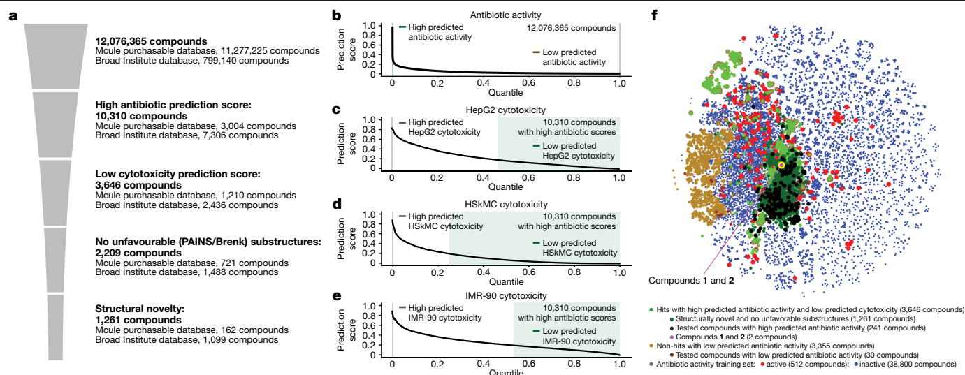
Fig. 2 | Filtering and visualizing chemical space. a , In silico filtering procedure. Trained graph neural networks are applied to make predictions of antibiotic activity for 12,076,365 compounds from the Mcule purchasable database and a Broad Institute database. Compounds with high (>0.4 for the Mcule database, and >0.2 for the Broad Institute database) prediction scores for antibiotic activity are retained, and similar graph neural networks are applied to predict the cytotoxicity of these compounds for HepG2 cells, HSKMCs, and IMR-90 cells. Compounds with low (<0.2) cytotoxicity prediction scores for all cell types are retained, then computationally tested for the presence of promiscuously reactive or unfavourable chemical substructures (PAINS and Brenk substructures). Finally, the remaining compounds are
