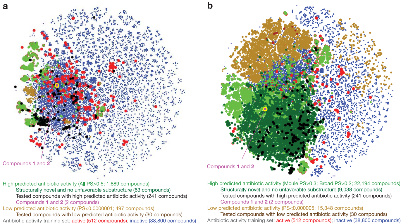
Extended Data Fig. 4 | Visualizing chemical space across different prediction score thresholds. a, b, t-Distributed neighbor embedding (t-SNE) plot of compounds with high and low antibiotic prediction scores, in addition to compounds in the training set, for different prediction score thresholds. The
