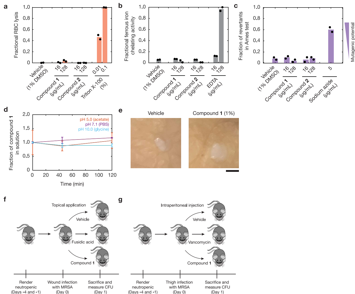
Extended Data Fig. 9 | Toxicity, chemical properties, and in vivo efficacy of compounds 1 and 2. a , Fractional hemolysis measurements of human red blood cells (RBCs) treated with compounds 1 and 2 at the indicated final concentrations. Vehicle (1% DMSO) was used as a negative control, and Triton X-100, a detergent, was used as a positive control. Black points indicate values from two biological replicates, and red bars indicate average values. b , Ferrous iron chelation measurements of compounds 1 and 2. Vehicle (1% DMSO) was used as a negative control, and ethylenediaminetetraacetic acid (EDTA), an iron chelator, was used as a positive control. Black points indicate values from two biological replicates, and gray bars indicate average values. c , Ames test mutagenesis measurements of the fractions of revertant S. typhimurium TA100 cultures treated with compounds 1 and 2 at the indicated final concentrations. Vehicle (1% DMSO) was used as a negative control, and 5 µg/mL sodium azide
