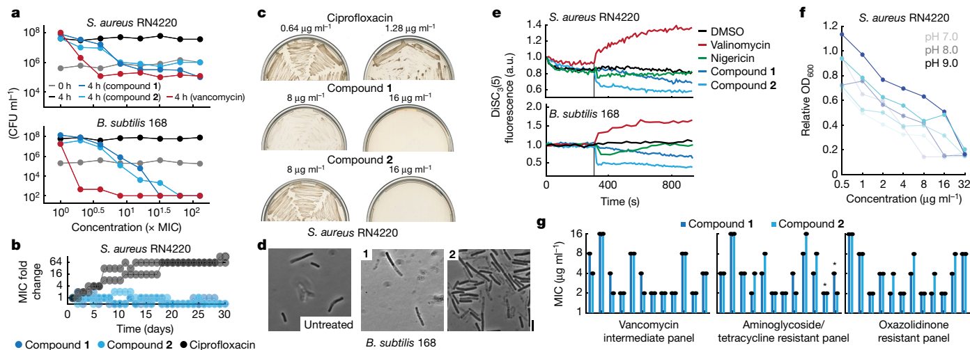
Fig. 4 | Resistance and mechanism of action of a structural class. a , Time-kill measurements for log-phase S. aureus RN4220 and B. subtilis 168 treated with compounds 1 and 2 , vancomycin or untreated. Data are from two biological replicates, and points indicate mean values. Where applicable, CFU per ml values less than 10^2 were truncated to a value of 10^2 to reflect the lower limit of quantification. b , MIC fold changes in serial passaging experiments, in which S. aureus RN4220 was passaged in liquid LB every 24 h for 30 days. Two biological replicates (individual curves) are shown for each compound, and fold change is on a log scale. c , Growth of suppressor mutants in evolution experiments, in which S. aureus RN4220 was plated at 10^9 CFU on LB agar plates containing compound, incubated for 5 days, then streaked on fresh compound-containing LB agar plates. Each image represents two biological replicates. d , Phase-contrast images of log-phase B. subtilis 168 cells treated with compounds 1 and
