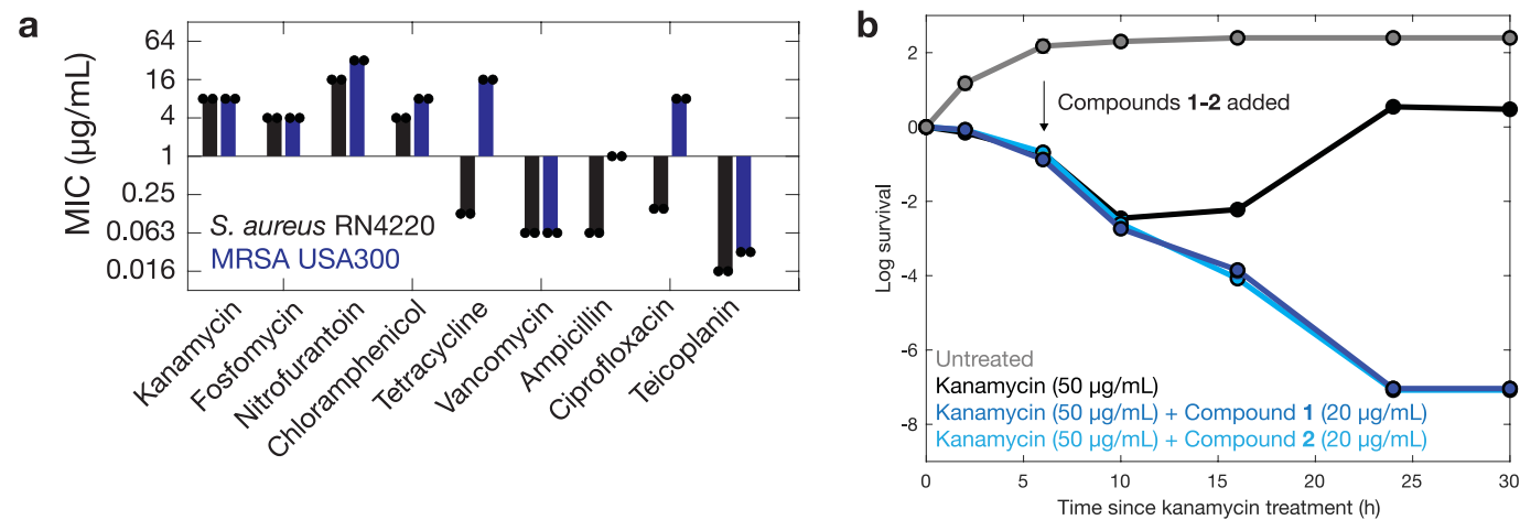
Extended Data Fig. 8 | Comparison of MICs of different compounds against methicillin-susceptible and methicillin-resistant S. aureus , and eradication of kanamycin persists by treatment with compounds 1 and 2. a , MICs of various antibiotics against S. aureus RN4220 (black) and S. aureus USA300 (blue) on a log scale. Bars show the mean of two biological replicates (individual points). b , Survival curves of B. subtilis 168 after combination treatment with
