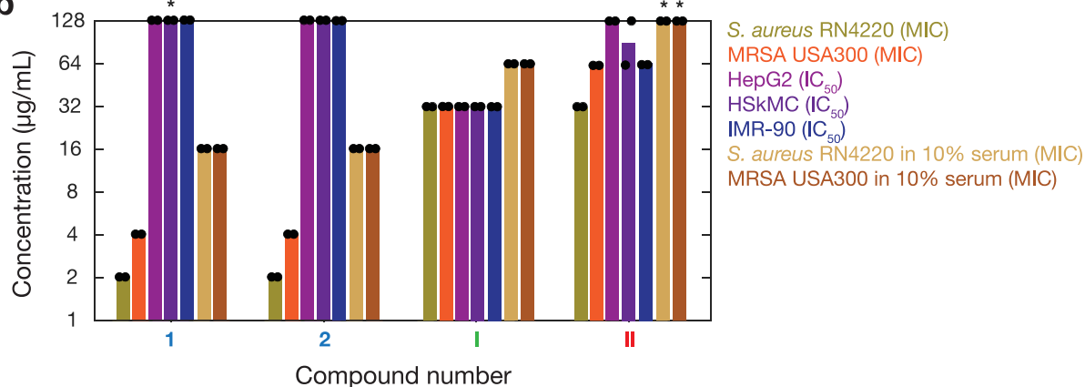
Extended Data Fig. 7 | Closest active training set compounds to, and selectivities of, four validated hits associated with rationale groups G1-G5.
