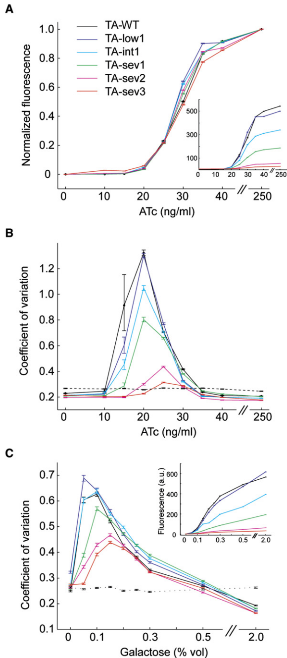
Figure 2. P_{GAL1^+} Transcriptional Activity and Population Heterogeneity at Varying Levels of ATc and Galactose
