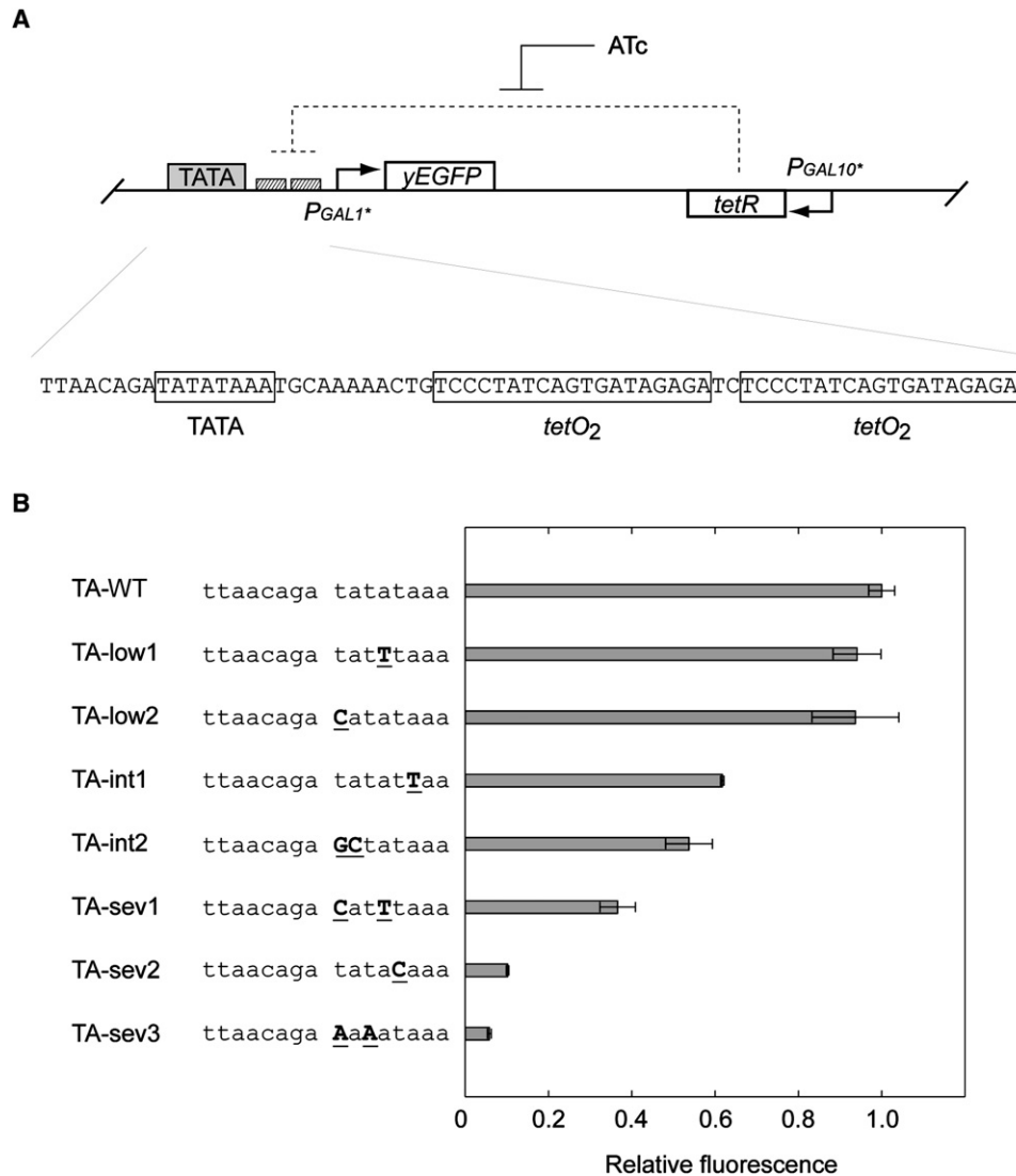
Figure 1. Engineered Expression Control and Variants of the GAL1 TATA Box
