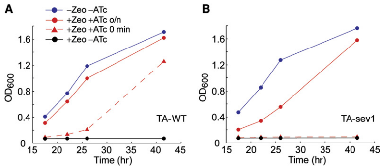
Figure 5. Effect of Promoter Response Time on Culture Growth after Exposure to Zeocin Antibiotic
