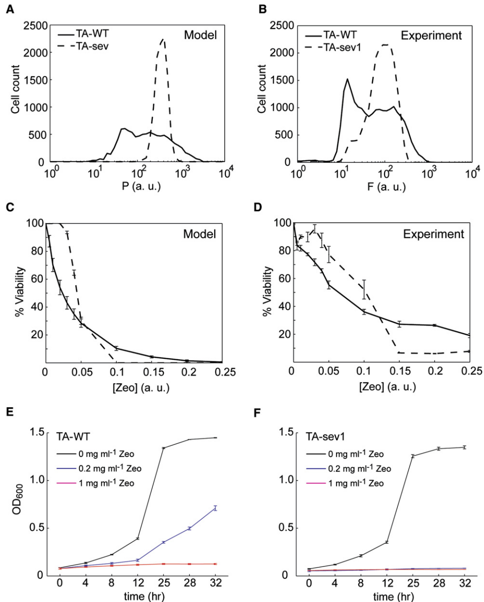
Figure 6. Phenotypic Benefit of Cell-Cell Heterogeneity upon Exposure to Zeocin Antibiotic
