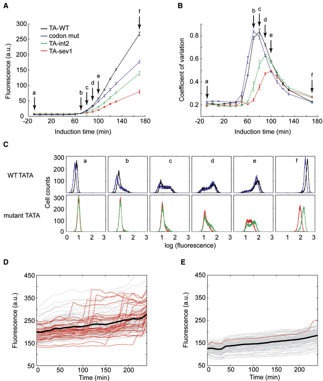
Figure 4. P_{GAL1^+} Induction and Heterogeneity of Response
