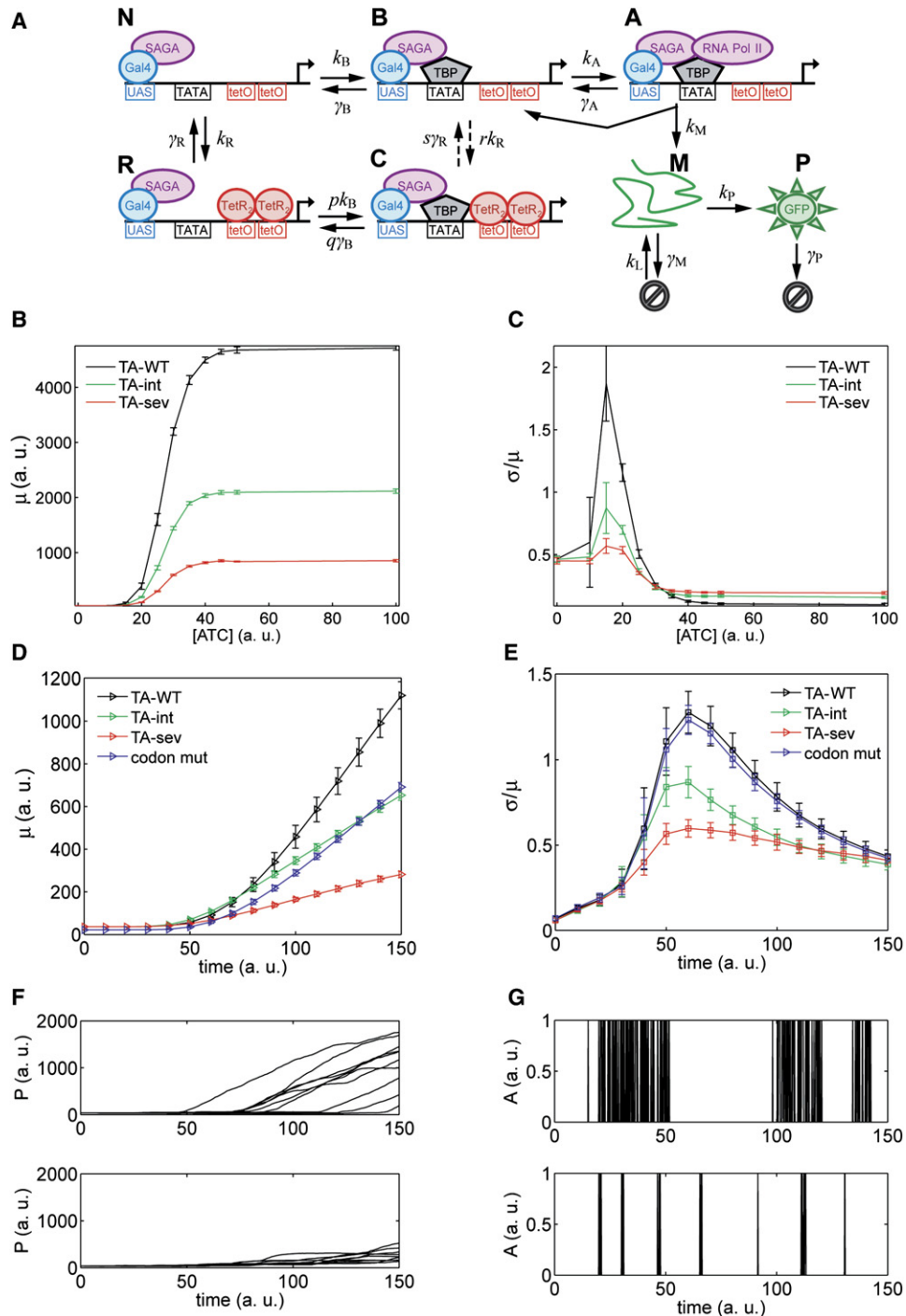
Figure 3. Modeling the Effects of Transcription Scaffold Stability on Gene Expression Variability
