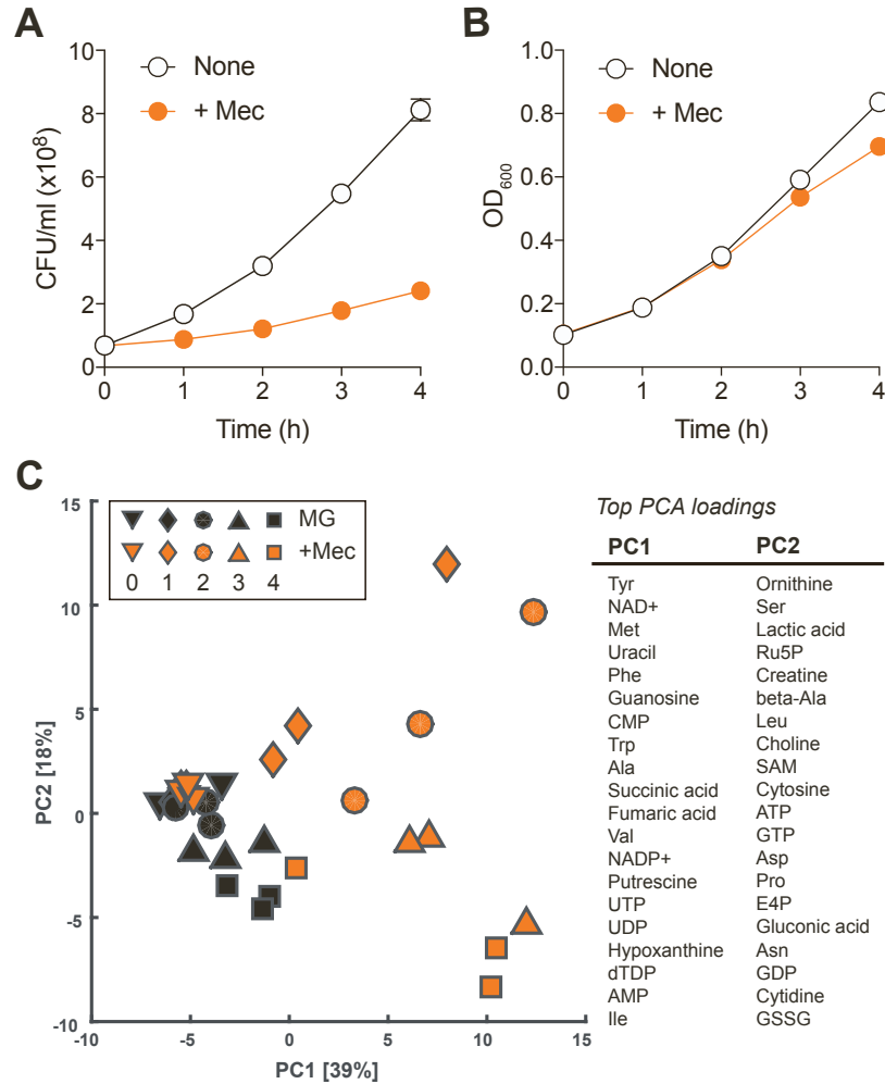
Figure S1. Mecillinam treatment induces broad shifts in the E. coli metabolome; related to Figure 1.
