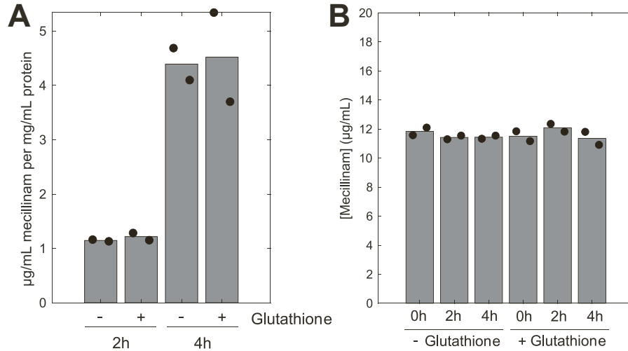
Figure S5. Glutathione does not impact mecillinam uptake or react with mecillinam; related to Figure 5.
