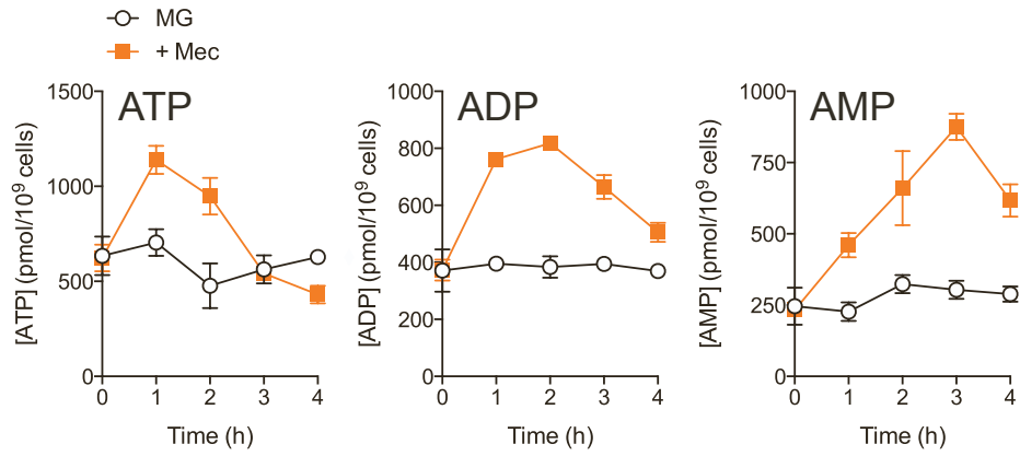
Figure S2. PBP2 inhibition induces temporal dynamic shifts in the adenylate energy system; related to Figure 2.
