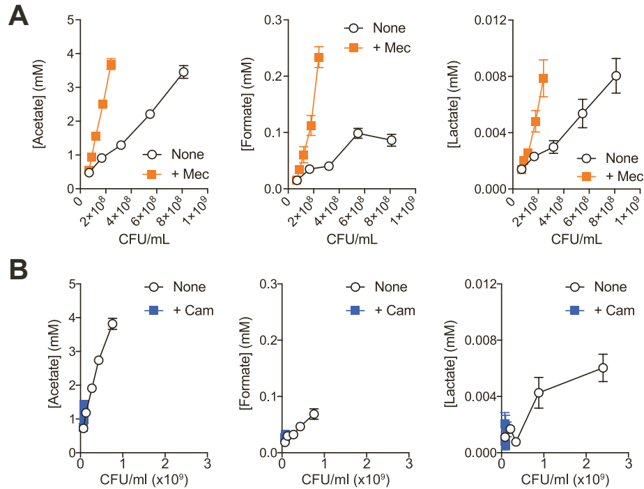
Figure S3. Mecillinam and chloramphenicol have disparate impacts on the secretion of mixed-acid fermentation products; related to Figure 2.
