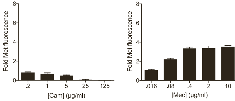
Figure S4. Mecillinam and chloramphenicol induce differing dose-responsive behaviors in protein translation; related to Figure 4.
